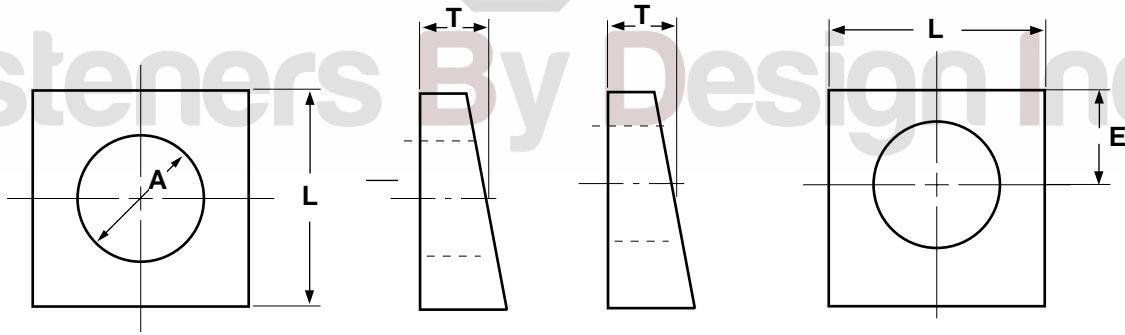
Square Beveled
