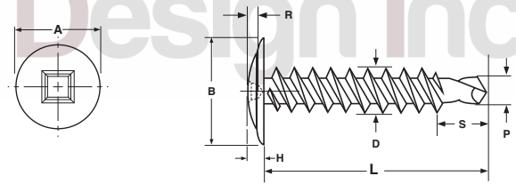
Square Recess
