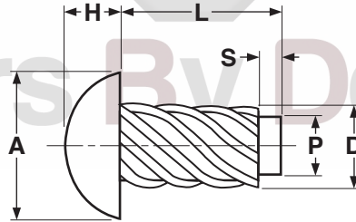
DRIVE SCREWS - ROUND HEAD TYPE U ASME B18.6.3-2013
