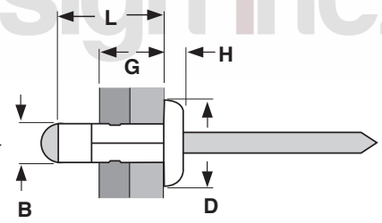
DOME HEAD
