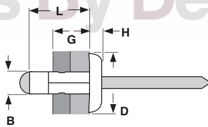
LARGE FLANGE
